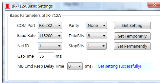
Figure 3-4 The basic settings window for IR-712A.
