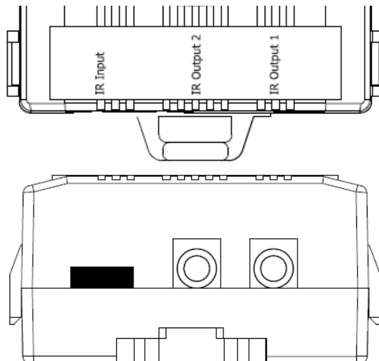
Figure 2-2 IR output 3.5 mm audio jack and learning input hole (front/bottom view).
