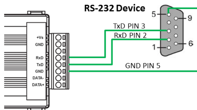
Figure 2-4 RS-232 wire connection.
