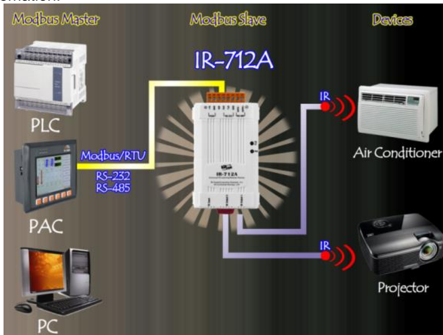
Figure 1-1 IR-712A application architecture.
