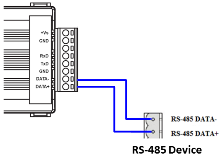
Figure 2-7 RS-485 wire connection.
