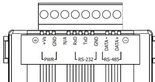
Figure 2-3 Screw terminal connector
