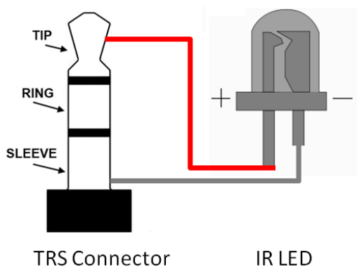
Figure 2-8 TRS connection
