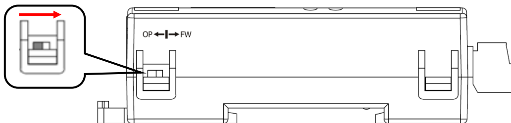
Figure 2-12 DIP switch in “FW” position.
