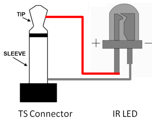
Figure 2-9 TS connection
