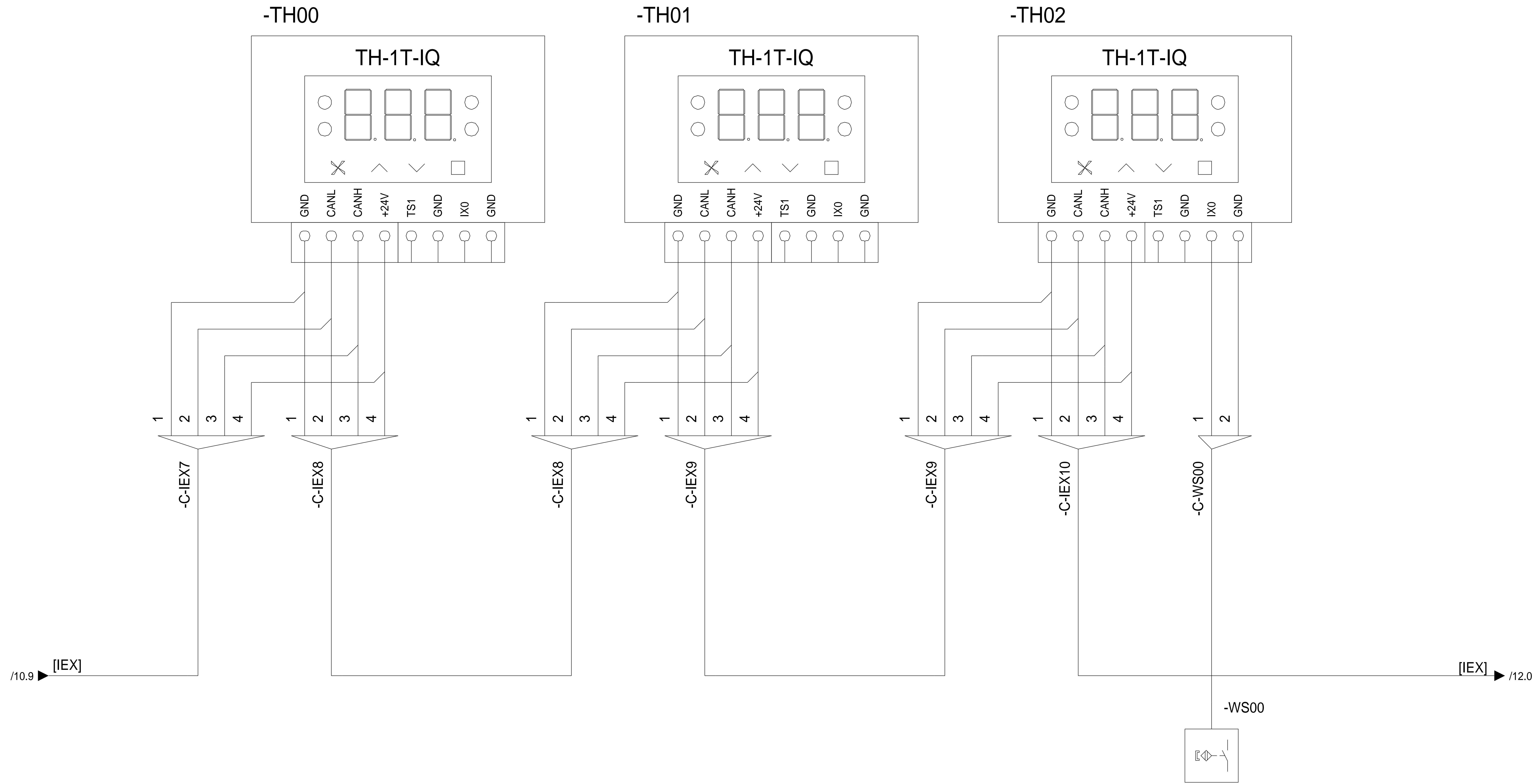
WINDOW SWITCH
